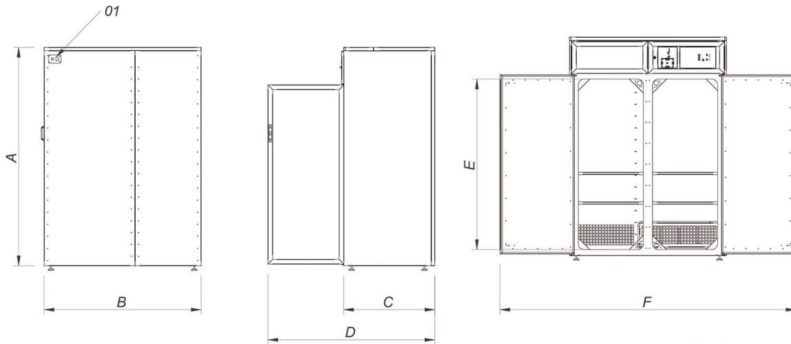
01. Power supply
