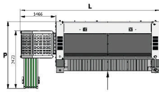
Standard stacker
